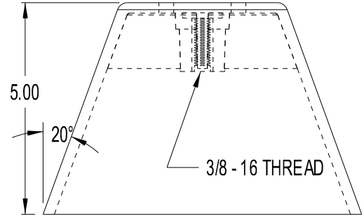
(OLD STYLE) ADAPTER PLUG PART # 3013 MATERIAL. - FILLED POLYPROPELENE
