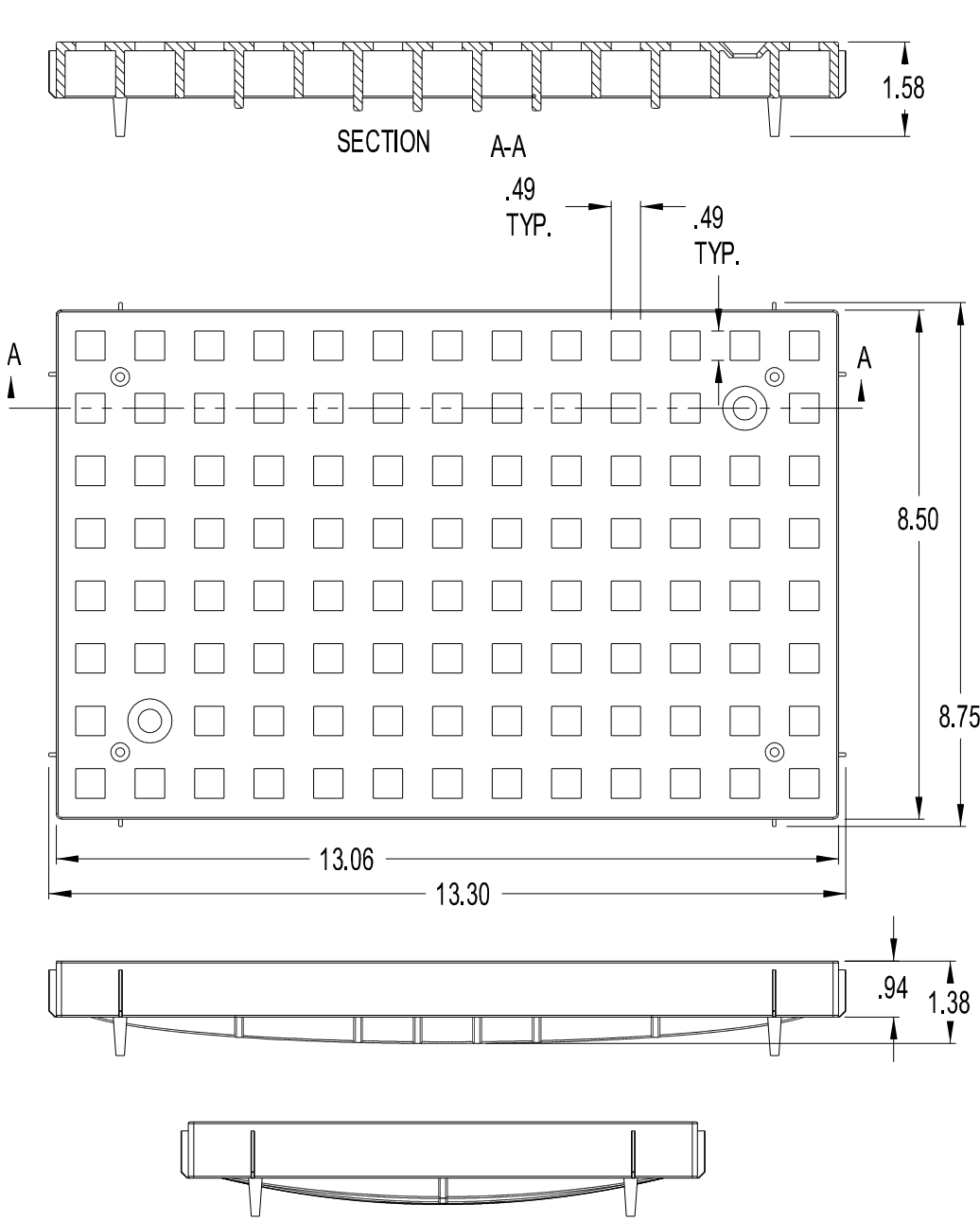
POLYLOK RAIN DRAIN GRATE PART NO. 3035 MATERIAL - FILLED POLYPROPYLENE
