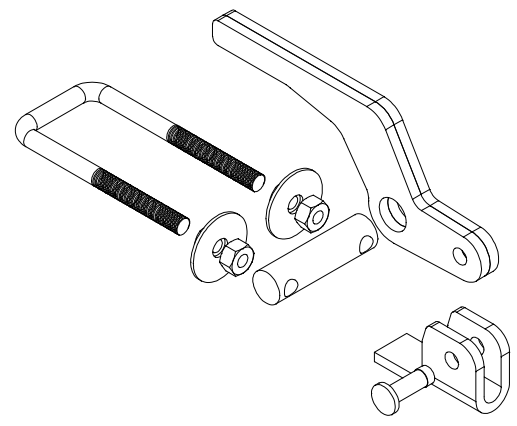
POLYLOK SMALL 6" D-BOX CLAMP PART NO. 3041 MATERIAL - A36 STEEL
