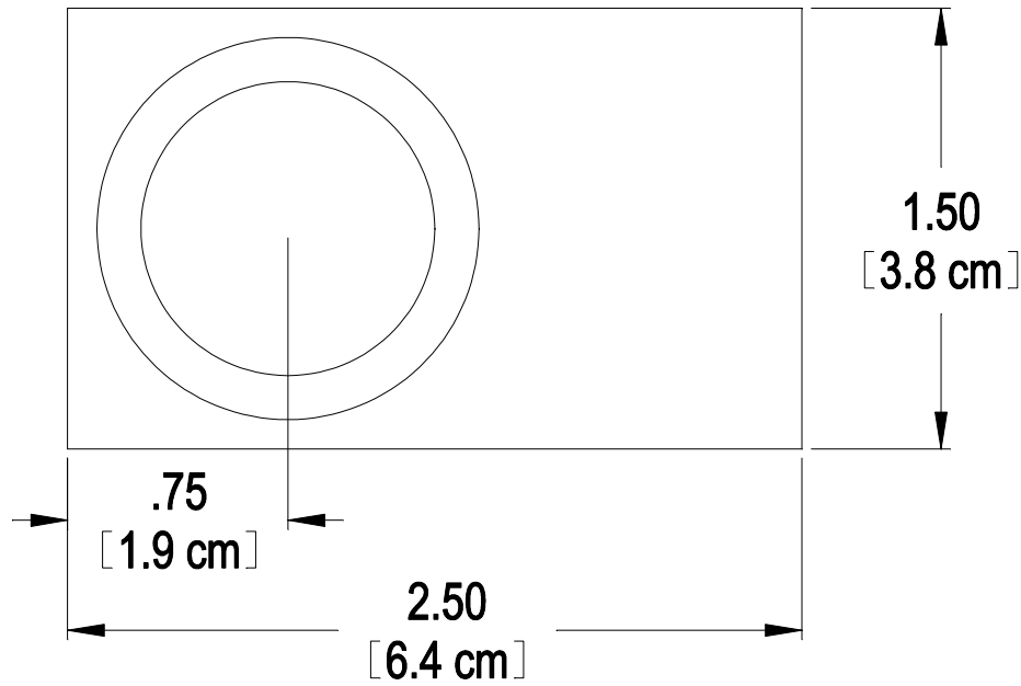
POLYLOK FORM CLAMP POST PART NO. 3043 MATERIAL - FORGED STEEL
