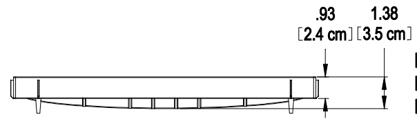
POLYLOK RAIN DRAIN GRATE (CAST IRON) PART NO. - 3035-1 MATERIAL - CAST IRON WEIGHT - 14 LBS
