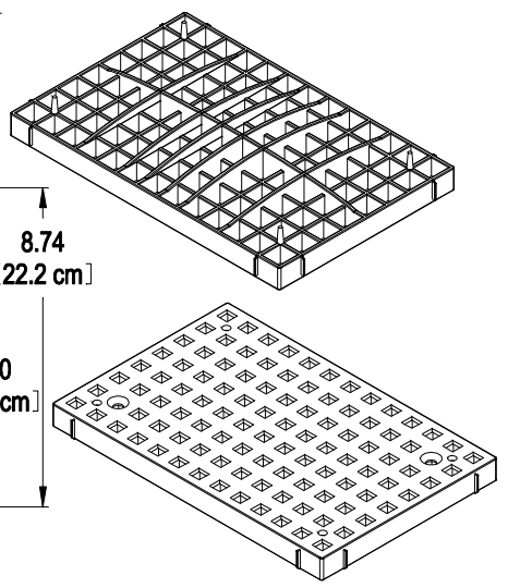
POLYLOK RAIN DRAIN GRATE PART NO. 3035 MATERIAL - FILLED POLYPROPYLENE
