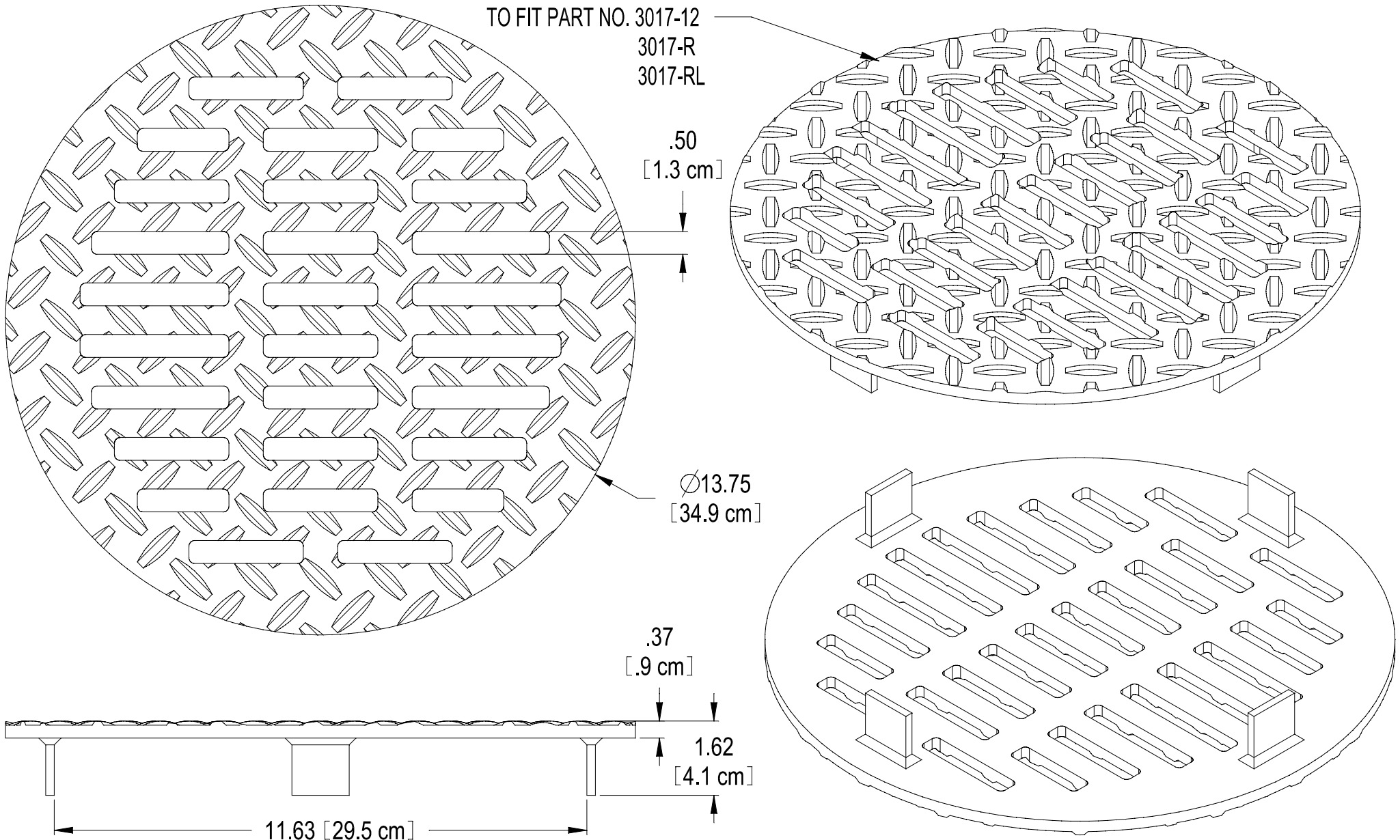
POLYLOK 12" METAL GRATE PART NO. 3017-M MATERIAL - GALVANIZED STEEL (DIAMOND PLATE)
