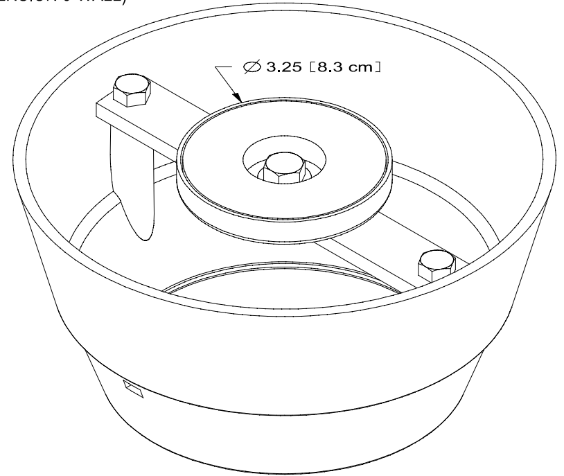
3022 MANDREL MAGNETIC MOUNT PART NO. 3022-MAG
