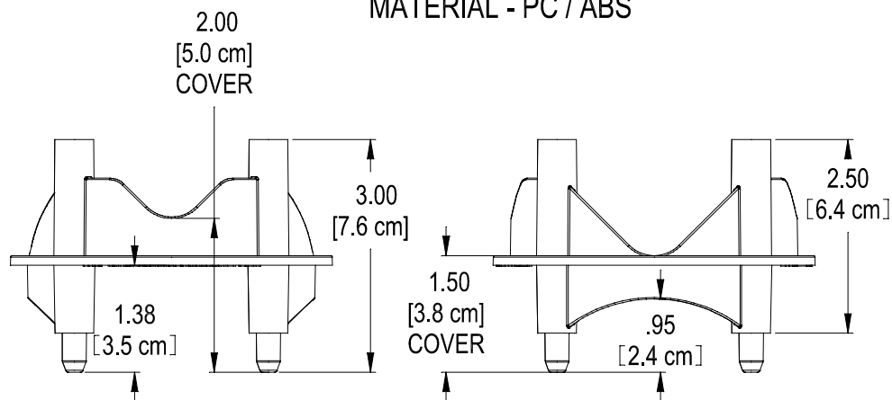
POLYLOK CHAIR 1.5" & 2" COVER PART NO. 3058-SC COLOR - GREY MATERIAL - PC / ABS
