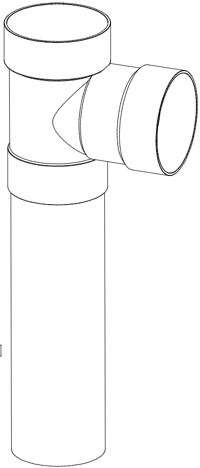
ASSEMBLED TEES PART NO. GDS-VT-B35 (SDR 35) GDS-VT-B40 (SCHD 40)
