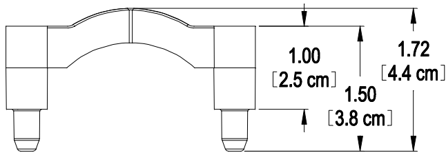
POLYLOK STACKING CHAIR SPACER PART NO. 3058-SS MATERIAL - REGRIND ABS
