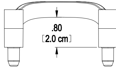
POLYLOK STACKING CHAIR SPACER PART NO. 3058-SS MATERIAL - REGRIND ABS
