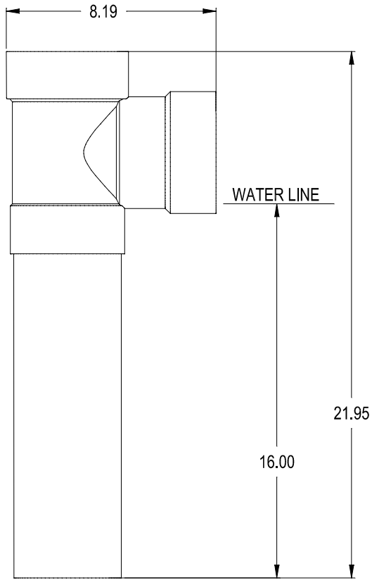
ASSEMBLED TEES PART NO. GDS-VT-B35 (SDR 35) GDS-VT-B40 (SCHD 40)
