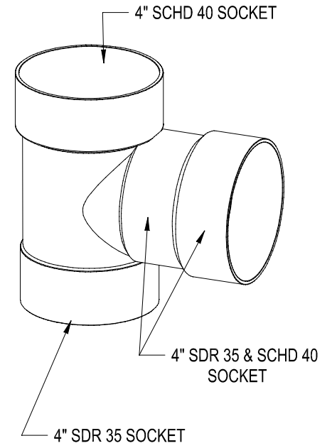
VERSA-TEE PART NO. GDS-VT
