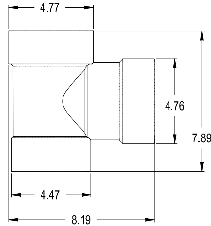
VERSA-TEE PART NO. GDS-VT
