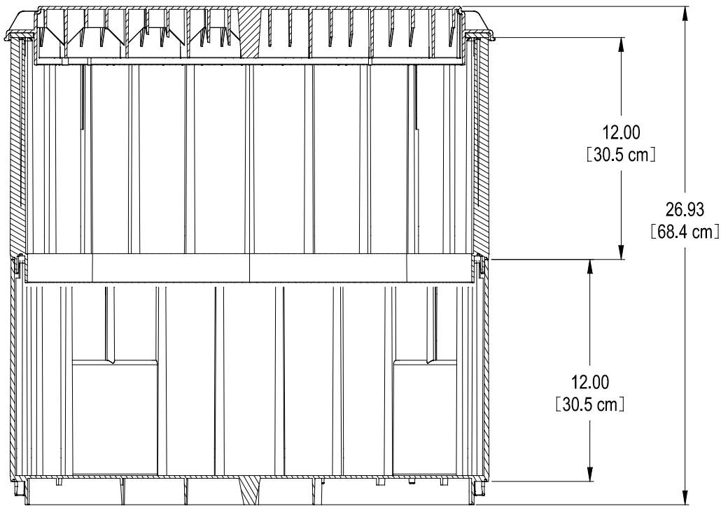
CUT - AWAY
