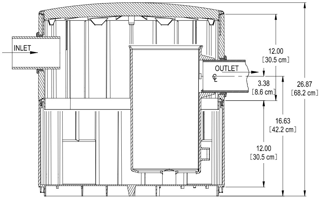
CUT - AWAY
