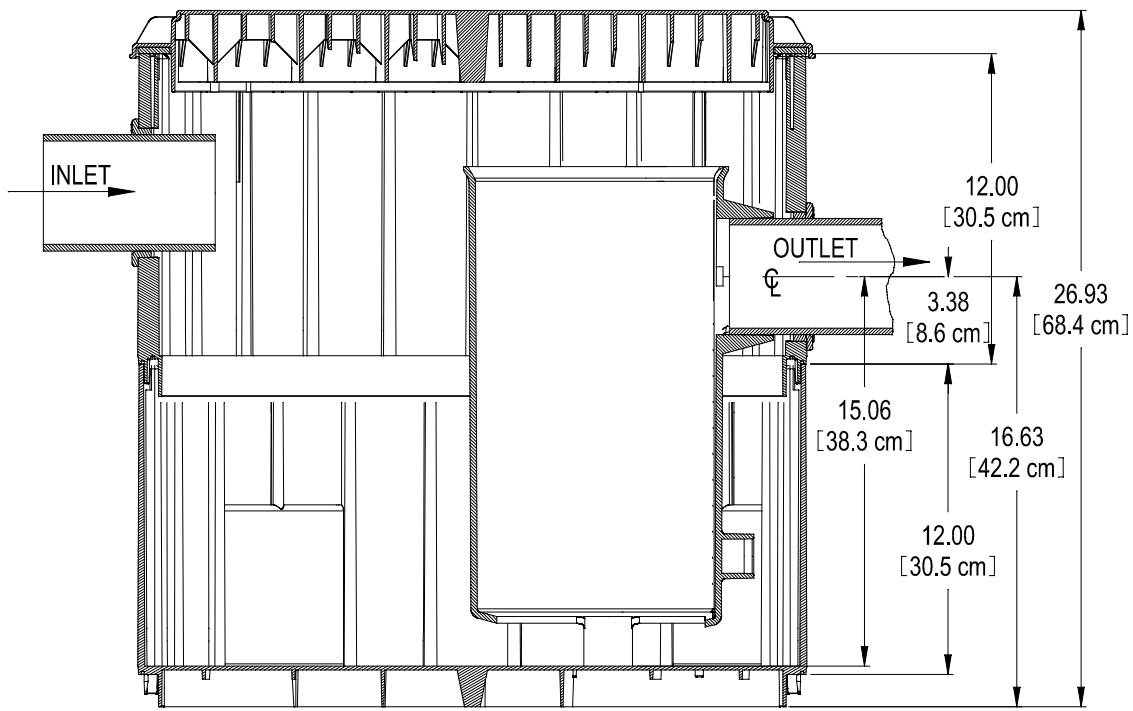
CUT - AWAY
