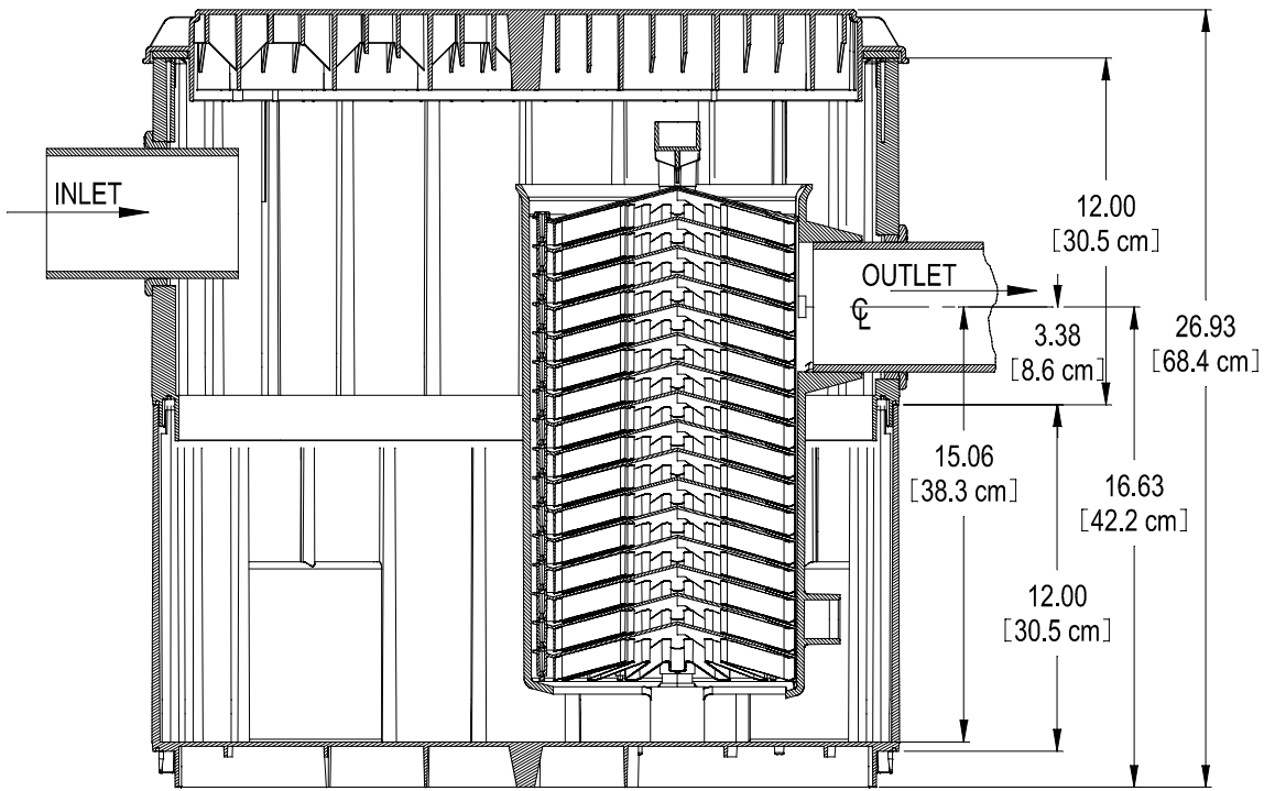
CUT - AWAY
