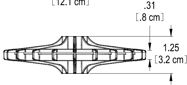
POLYLOK 1 1/2" COVER WHEEL PART NO. 30542 MATERIAL - HDPE ACCEPTS - 3-6 REBAR
