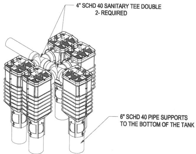
POLYLOK PL-525 5-GANG INSTALLATION
