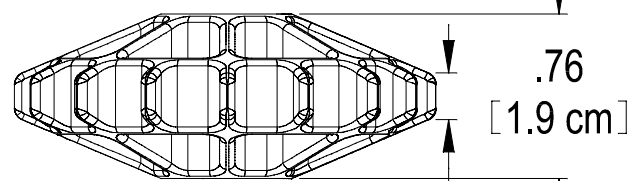
POLYLOK 7/8" WHEEL PART NO. 3053 MATERIAL - HDPE
