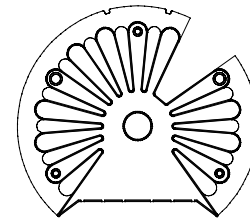
FILTER PLATE 8.15' (2.48 METERS) OF FILTRATION PER FILTER PLATE
