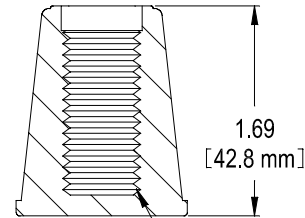
POLYLOK 5/8" THREADED INSERT PART NO. 30382-45T MATERIAL - ZINC ALLOY
