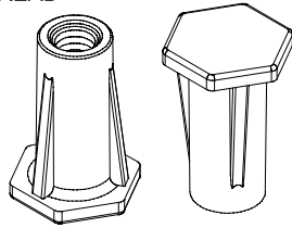
POLYLOK 3/8" THREADED INSERT PART NO. 30381-25T MATERIAL - ZINC ALLOY
