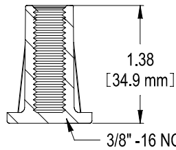
POLYLOK 3/8" THREADED INSERT PART NO. 30381-25T MATERIAL - ZINC ALLOY
