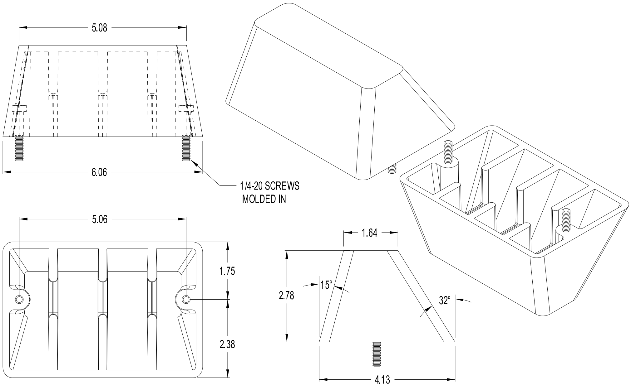
POLYLOK UNEQUAL KNOCKOUT OLD STYLE PART NO. 3044 MATERIAL - FILLED POLYPROPYLENE
