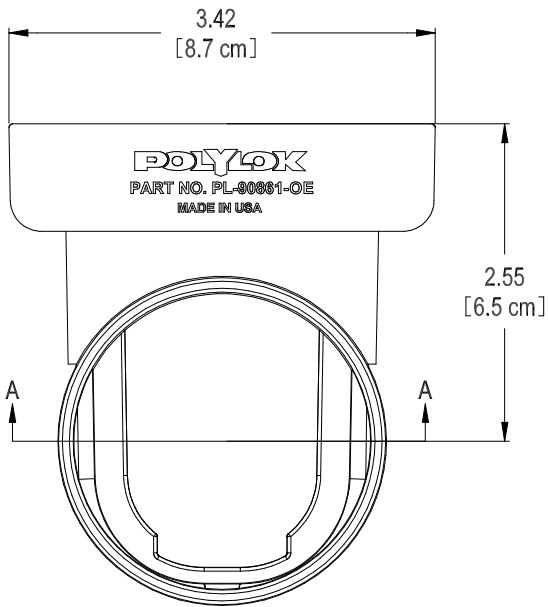
POLYLOK THIN TRENCH DRAIN OUTLET END PART NO'S. PL-90861-OE (BLACK) PL-90861-OEG (GREY) MATERIAL - ABS COLOR - BLACK, GREY
